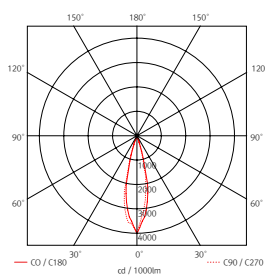
DVP3 40K-24V-POLE-BK-28-RP
