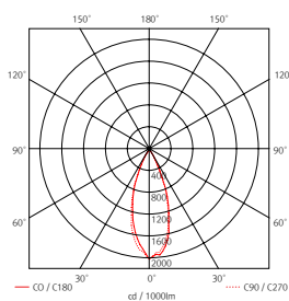
DVP3 40K-24V-POLE-BK-40-RP
