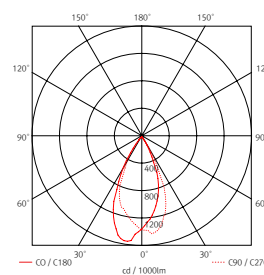
DVP3 40K-24V-POLE-BK-50-RP
