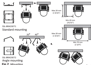
Fig.2 Mounting
